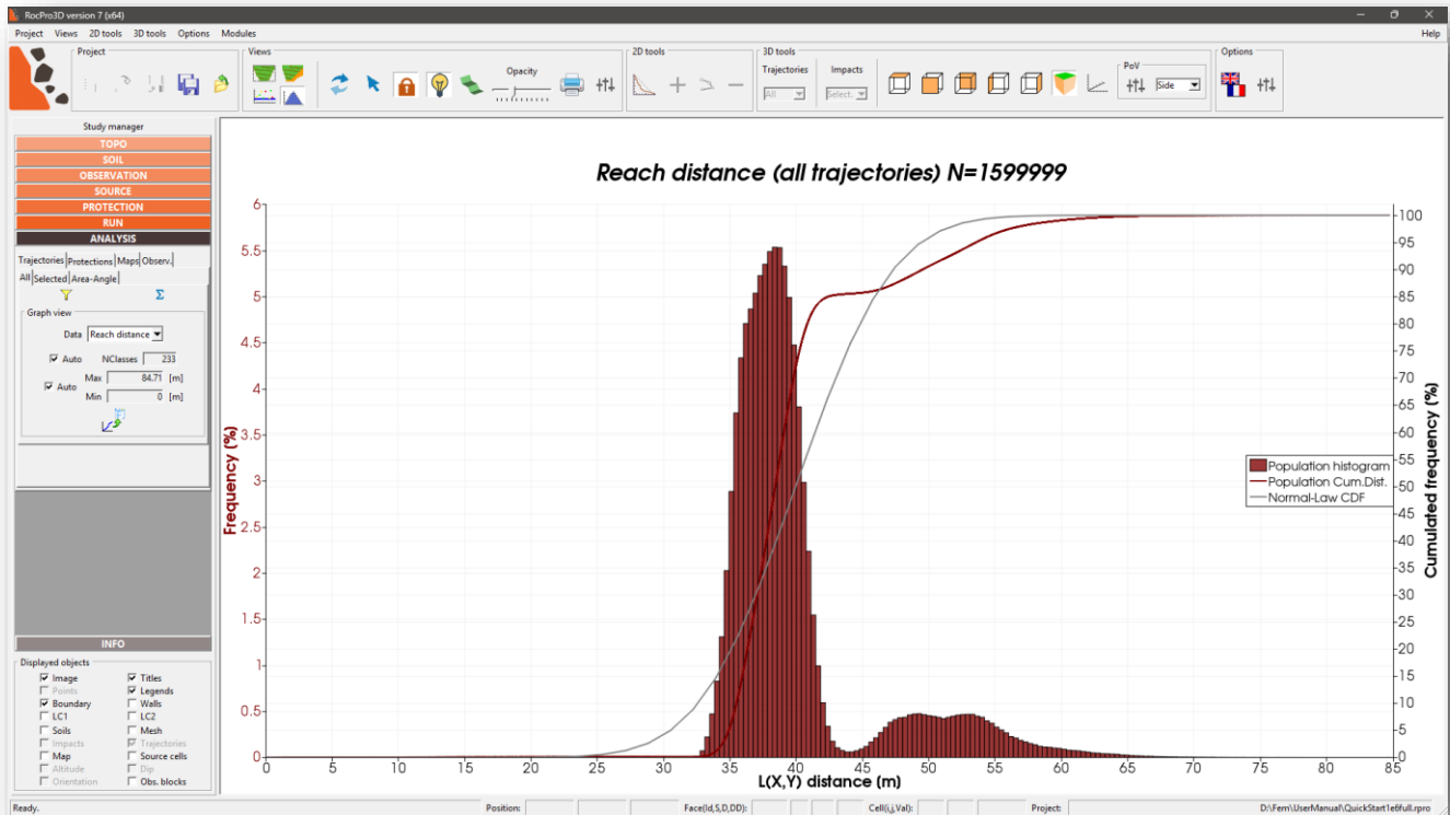
Histogram of the blocks reached distance [simulation with 1.6 \cdot 10^6 blocks]
